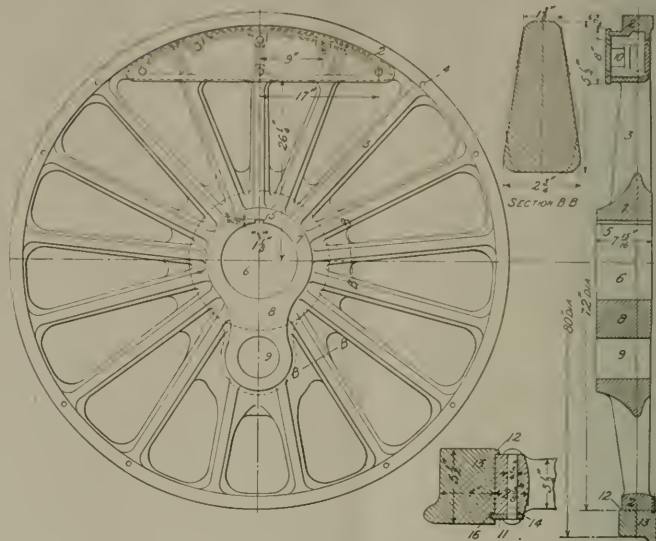
TRAILING DRIVING WHEEL.
